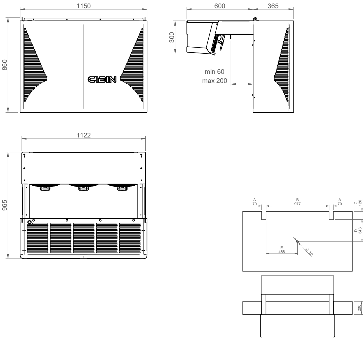
measurements for installing the monoblock
