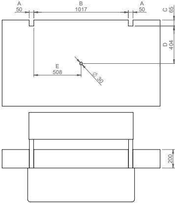
measurements for installing the monoblock
