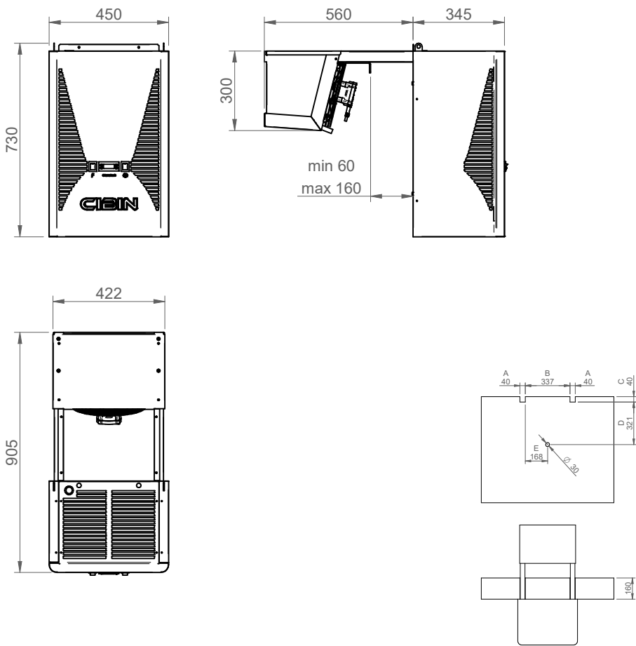
measurements for installing the monoblock
